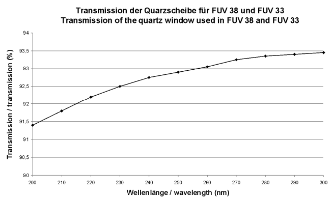
Transmission of the quartz window for all FUV
